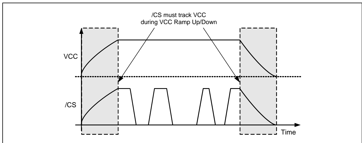
Figure 30b. Power-up, Power-Down Requirement
