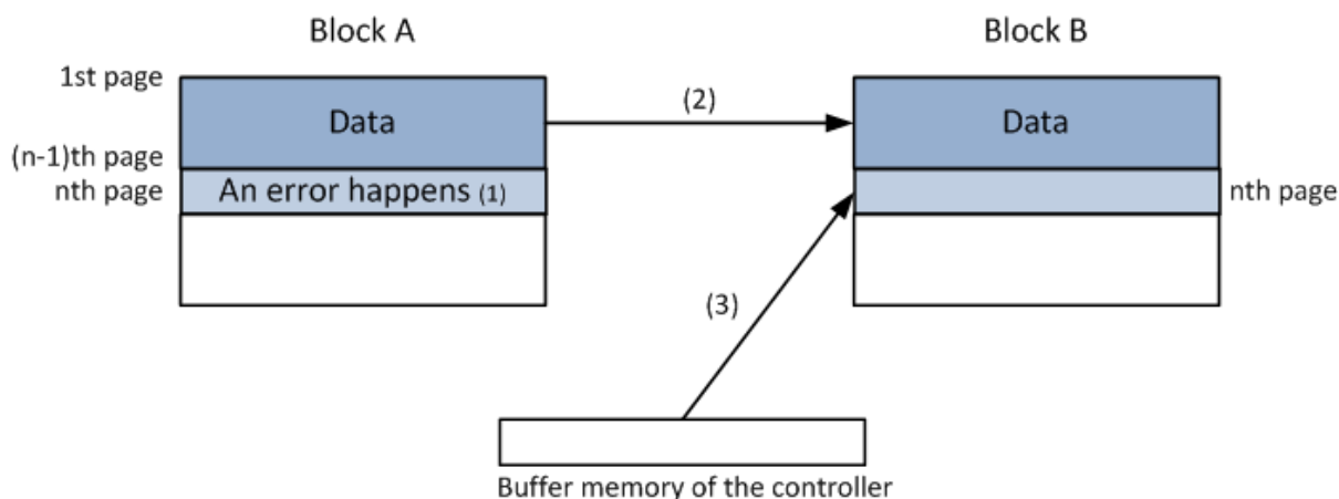
Figure 32. Bad Block Replacement
