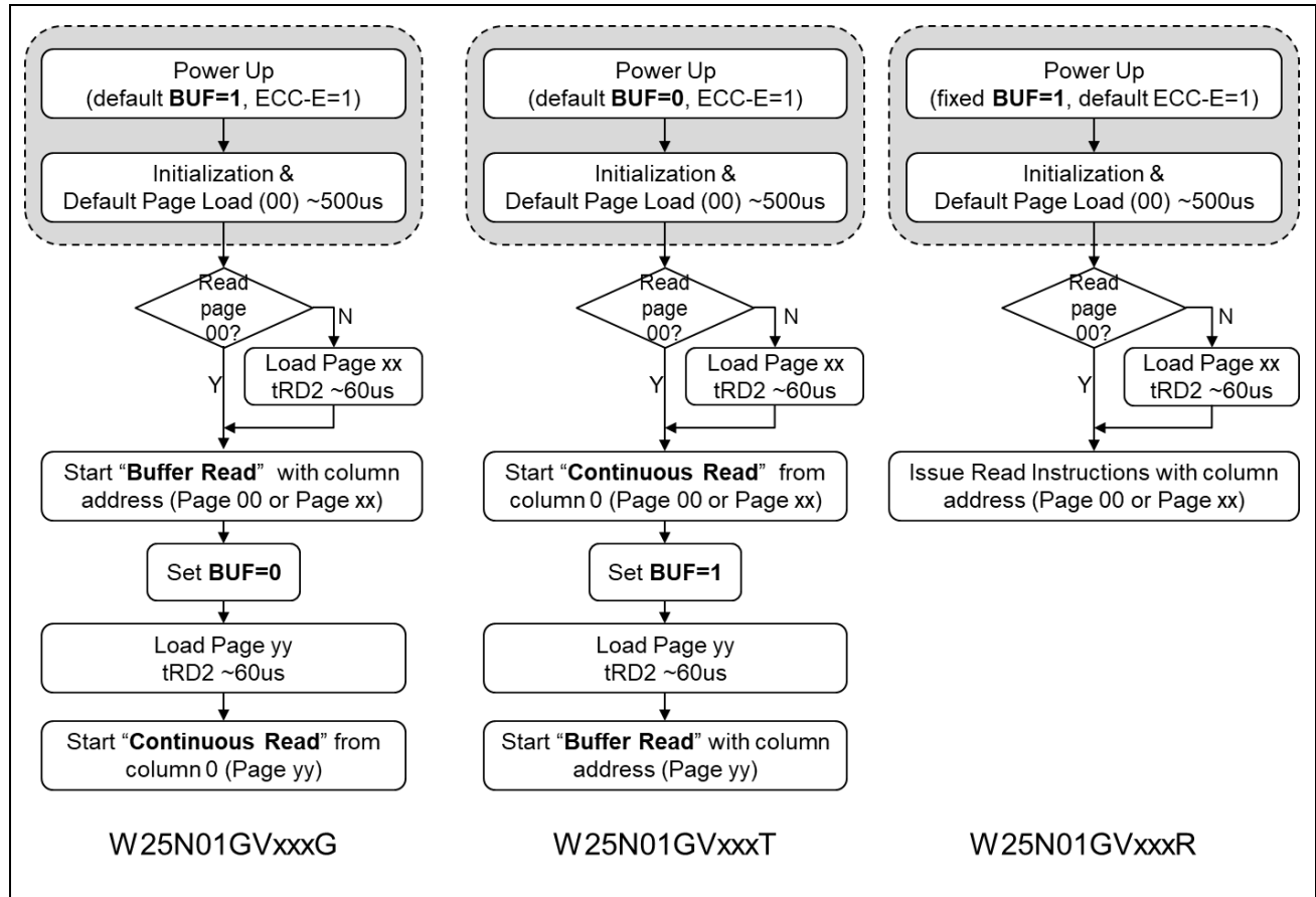
Figure 3. W25N01GV Flash Memory Operation Diagram
